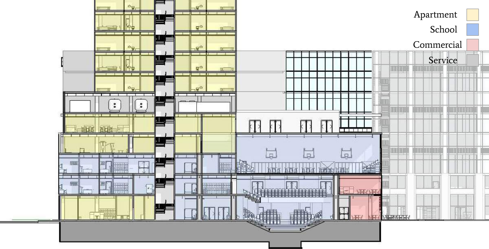
Longitudinal Section - Through School and Apartment
