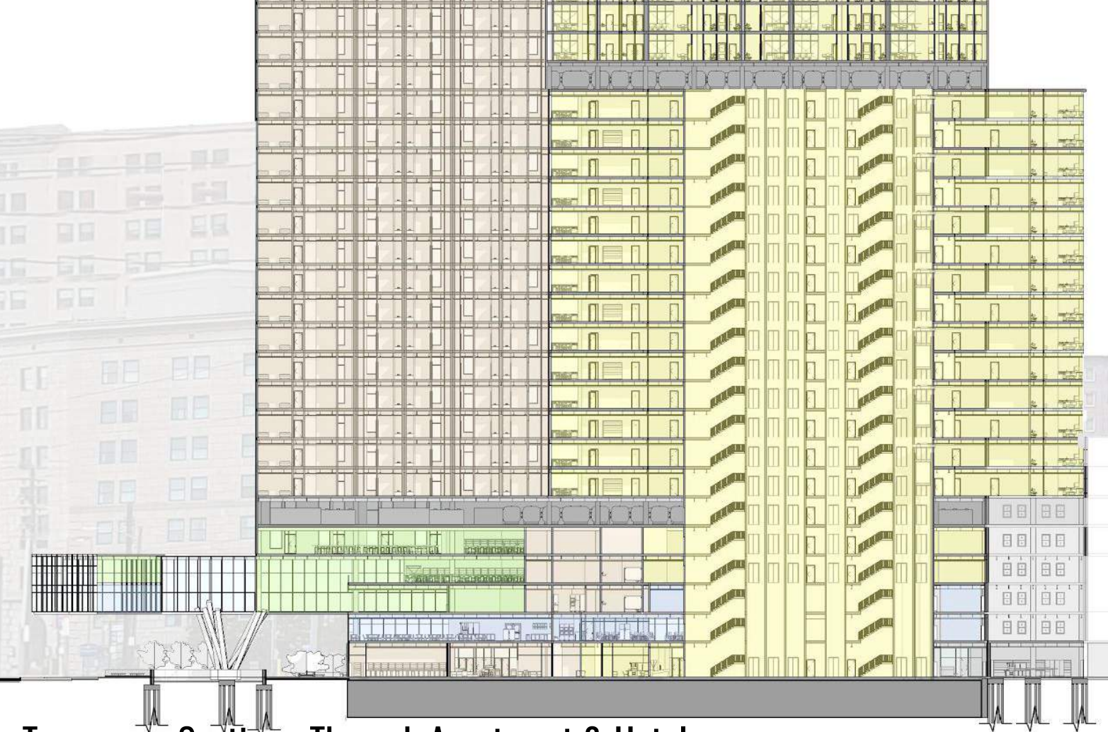
Transverse Section - Through Apartment & Hotel
